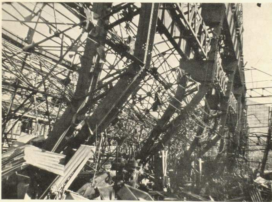
Photo No. 12. NAGASAKI. Large steel framed shed in the Mitsubishi Steel Works, \frac{1}{4} mile from the centre of damage. The steel stanchions have been bent (away from the explosion) and the roof trusses on both sides of these stanchions have collapsed. See paragraphs 22 and 32.
