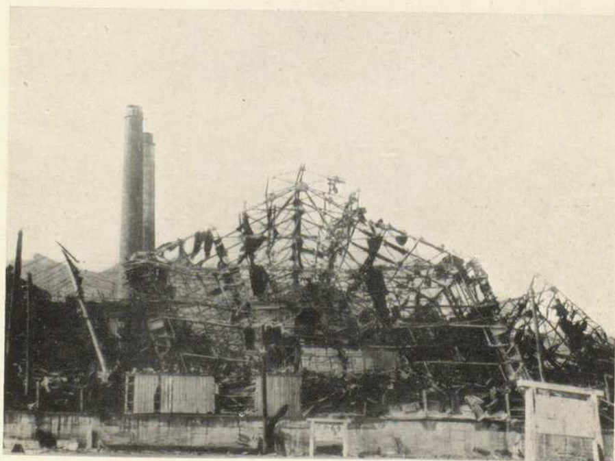
Photo No. 6. NAGASAKI. Mass distortion of steel framed shed buildings about half a mile from the centre of damage, which was to the right of the buildings in the photograph. It will be seen that the entire main frame is seriously distorted away from the explosion. See paragraphs 15, 22 and 32,
